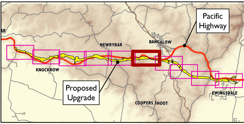
Figure 5.2f Proposed Upgrade Detail
