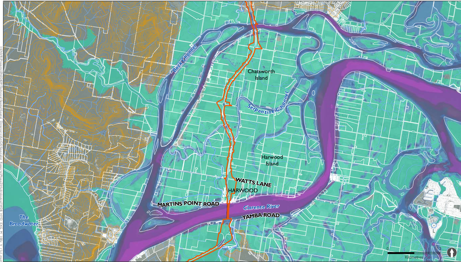
Figure 4-27 Peak 20y ARI flood velocities: Clarence River at Chatsworth and Harwood islands
