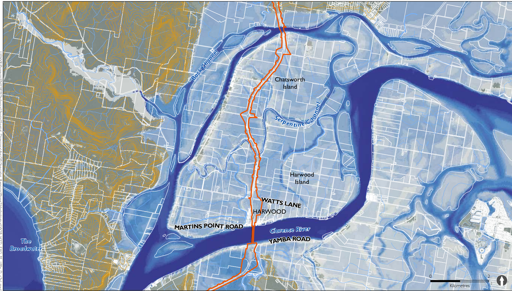
Figure 4-26 Peak 20 year ARI flood depths: Clarence River at Chatsworth and Harwood islands
