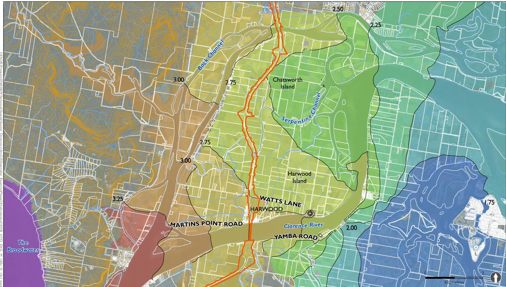
Figure 4-25 Peak 20 year ARI flood levels: Clarence River at Chatsworth and Harwood islands
