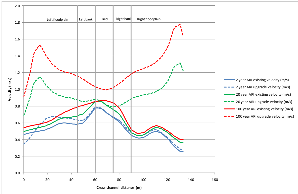
Figure H-5 Velocity profile of bridge at station 42.54
