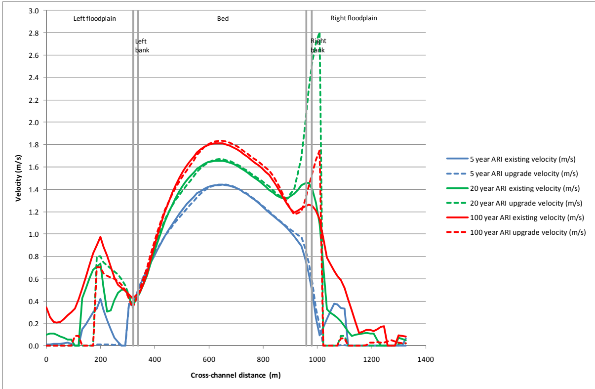
Figure H-17 Velocity profile of Harwood Bridge at station 85.60
