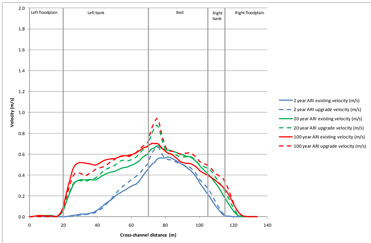
Figure H-19 Velocity profile of Tabbimoble Creek bridge at station 101.54
