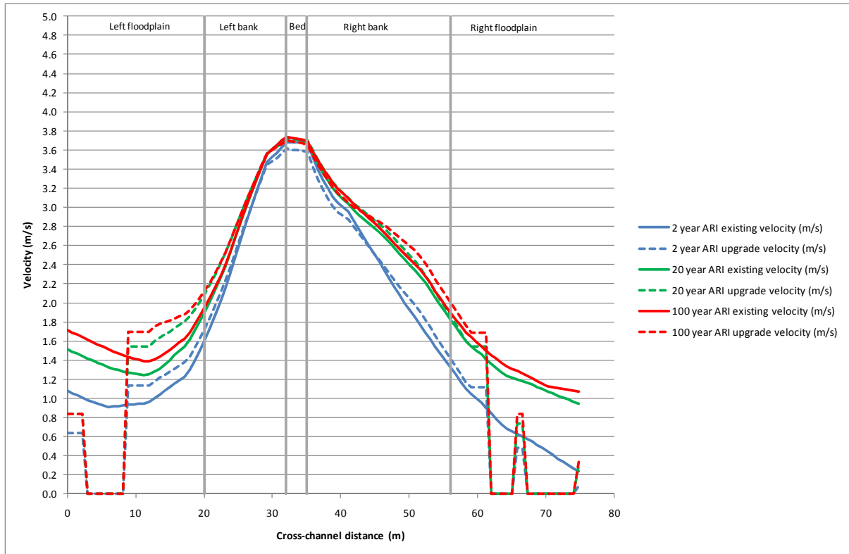
Figure H-9 Velocity profile of bridge over Black Snake Creek at station 46.67
