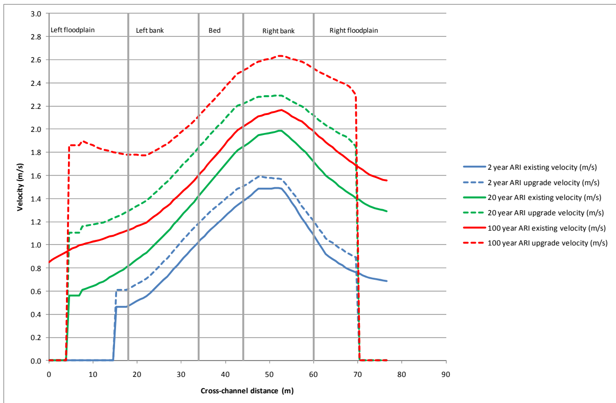
Figure H-12 Velocity profile of bridge over Chaffin Creek at station 52.44
