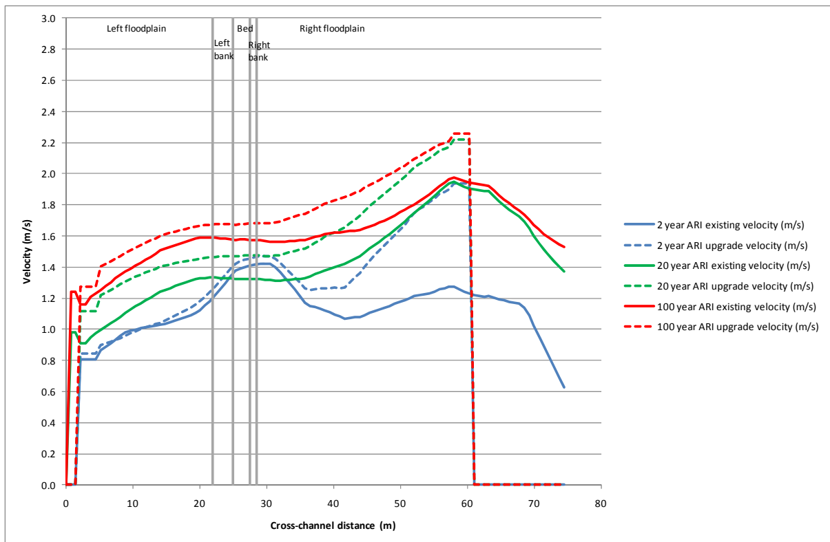
Figure H-10 Velocity profile of bridge at station 47.66
