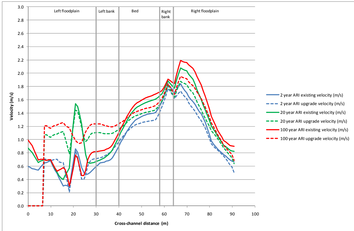
Figure H-1 Velocity profile of bridge over Corindi River at station 3.55
