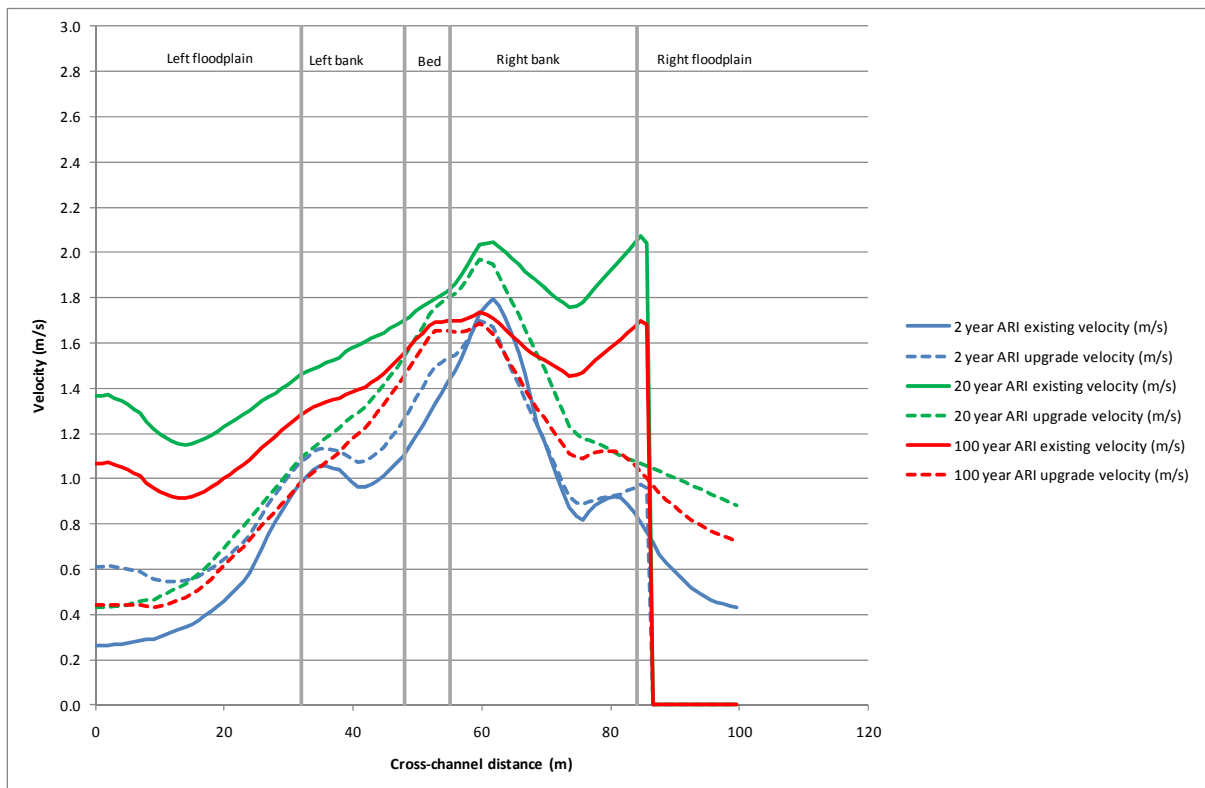
Figure H-8 Velocity profile of bridge over Pillar Valley Creek at station 46.34
