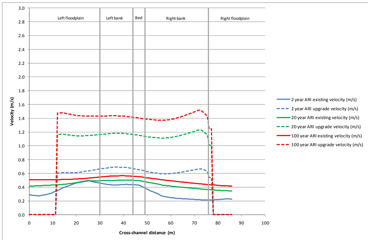
Figure H-14 Velocity profile of bridge over Champions Creek at station 57.03
