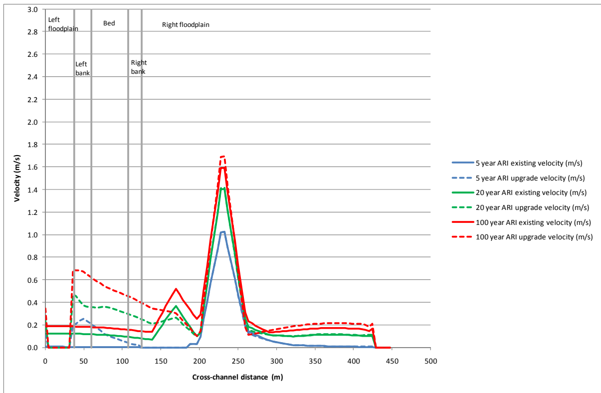
Figure H-16 Velocity profile of bridge over Shark Creek at station 74.76
