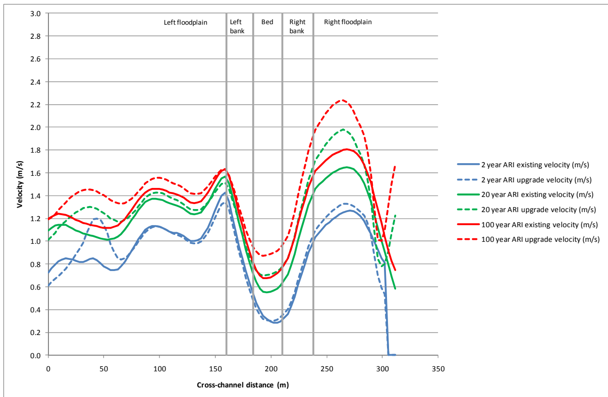
Figure H-6 Velocity profile of bridge over Coldstream River at station 43.12
