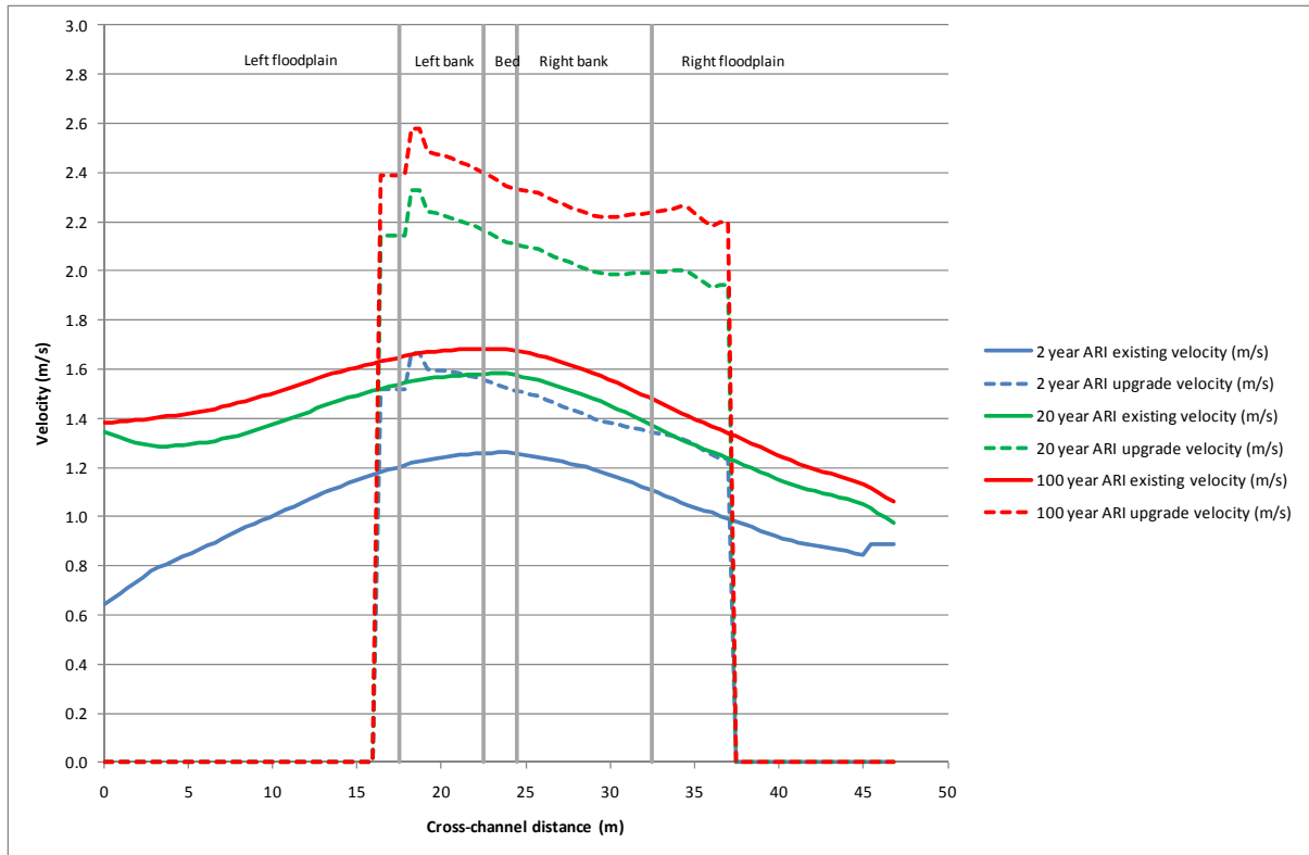
Figure H-11 Velocity profile of bridge at station 50.30
