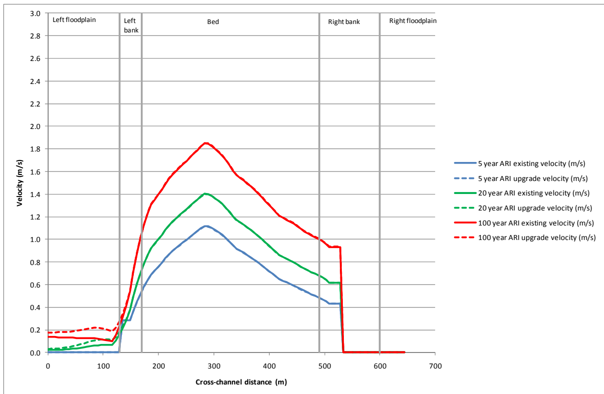
Figure H-22 Velocity profile of bridge over Richmond River at station 145.29
