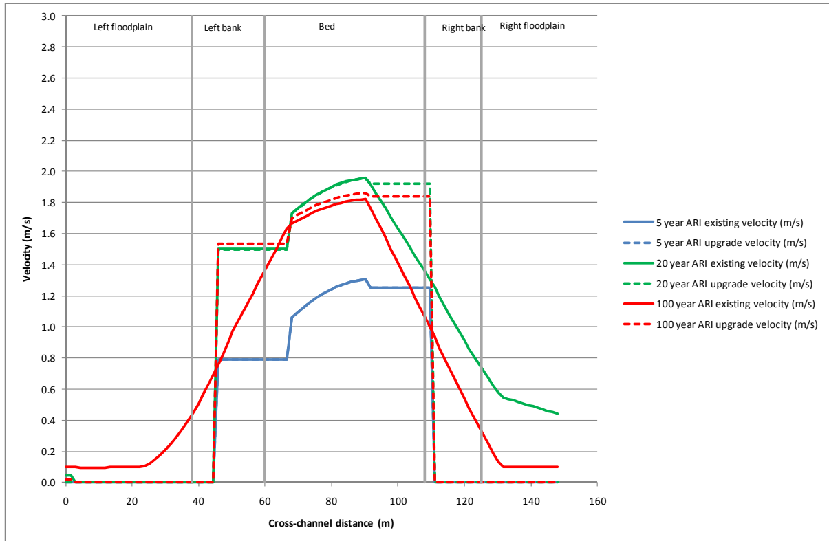
Figure H-21 Velocity profile of bridge over Tuckombil Canal at station 130.11
