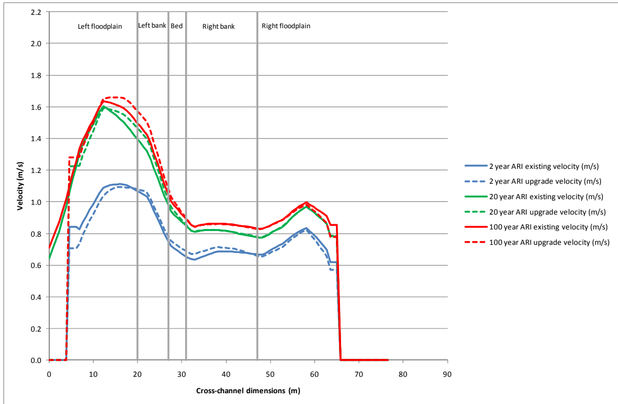
Figure H-15 Velocity profile of bridge at station 58.64
