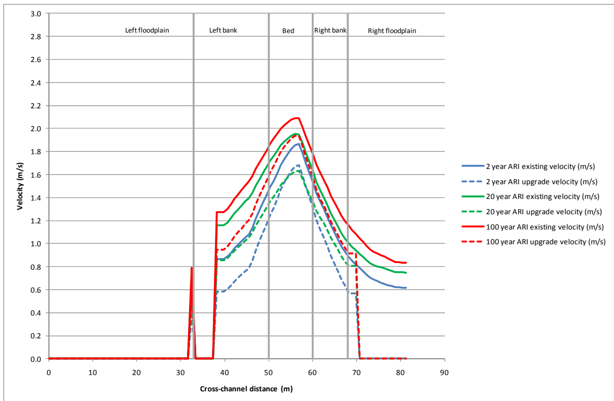
Figure H-4 Velocity profile of bridge over Pheasant Creek at station 36.40
