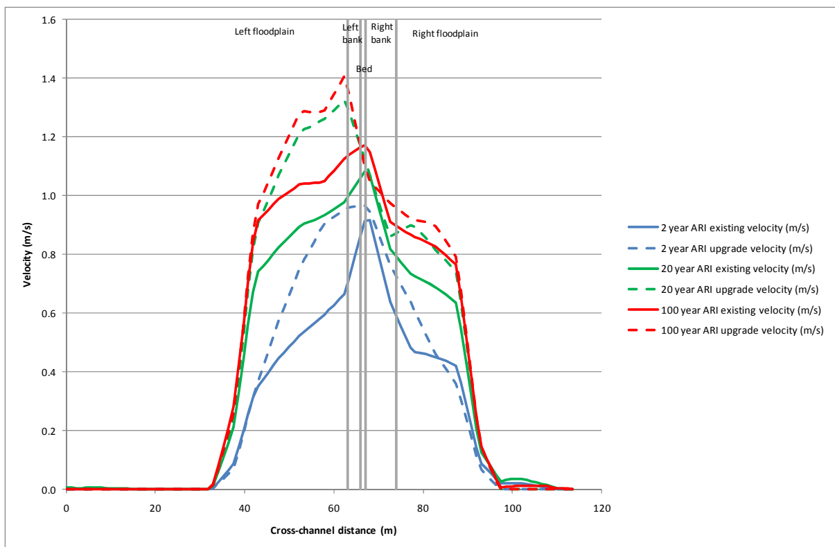
Figure H-20 Velocity profile of bridge at station 102.85
