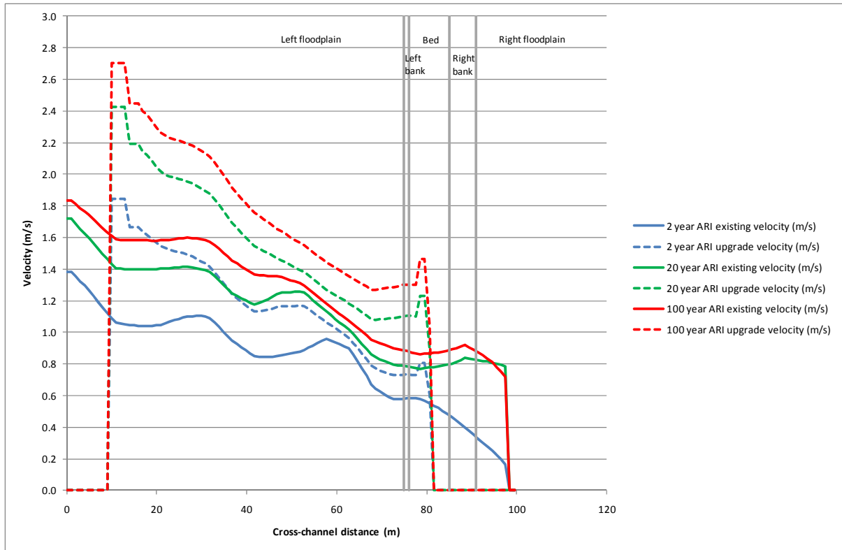
Figure H-13 Velocity profile of bridge at station 54.71
