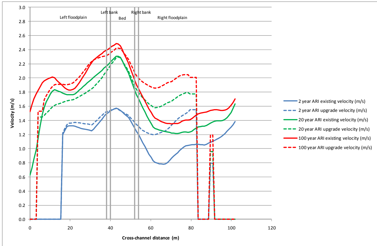
Figure H-7 Velocity profile of bridge at station 46.07
