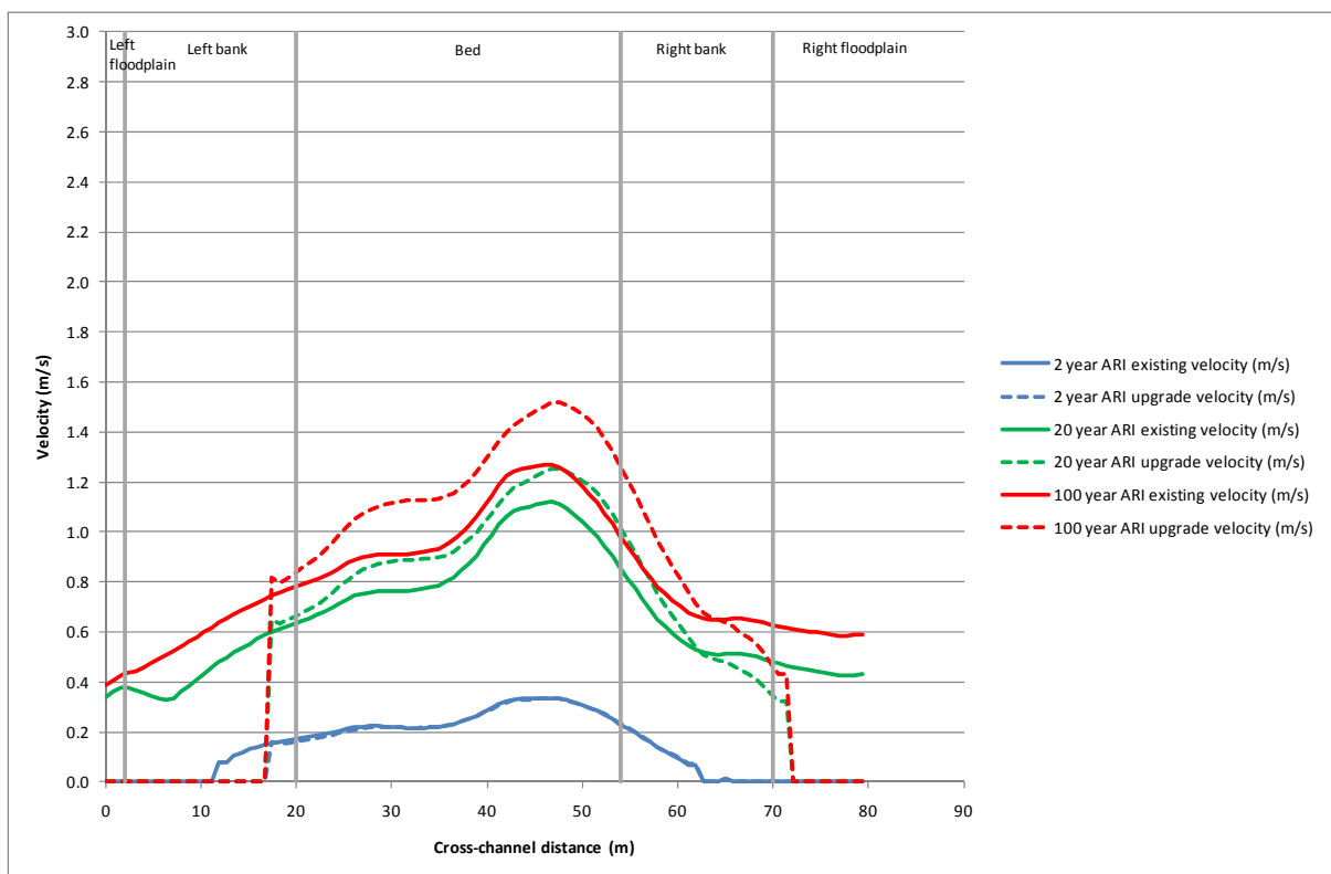
Figure H-2 Velocity profile of bridge over Cassons Creek at station 4.69
