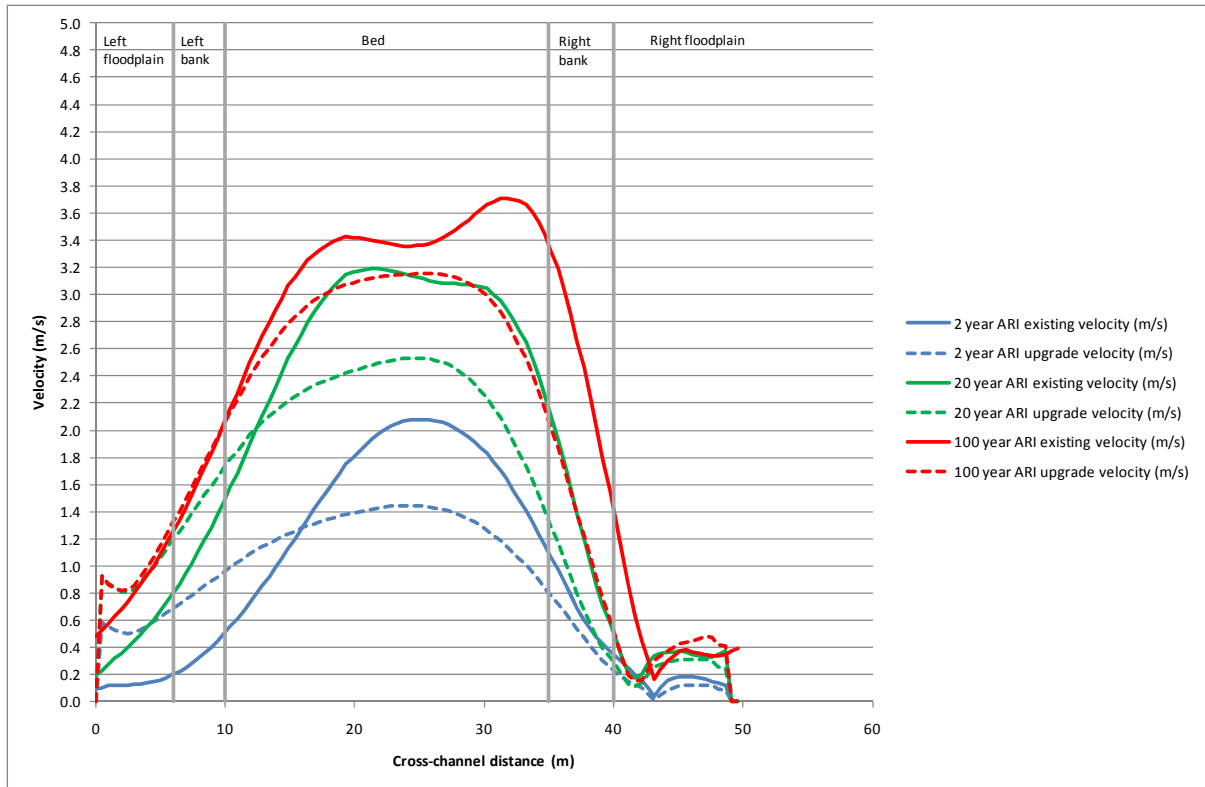
Figure H-3 Velocity profile of bridge over Halfway Creek at station 20.72
