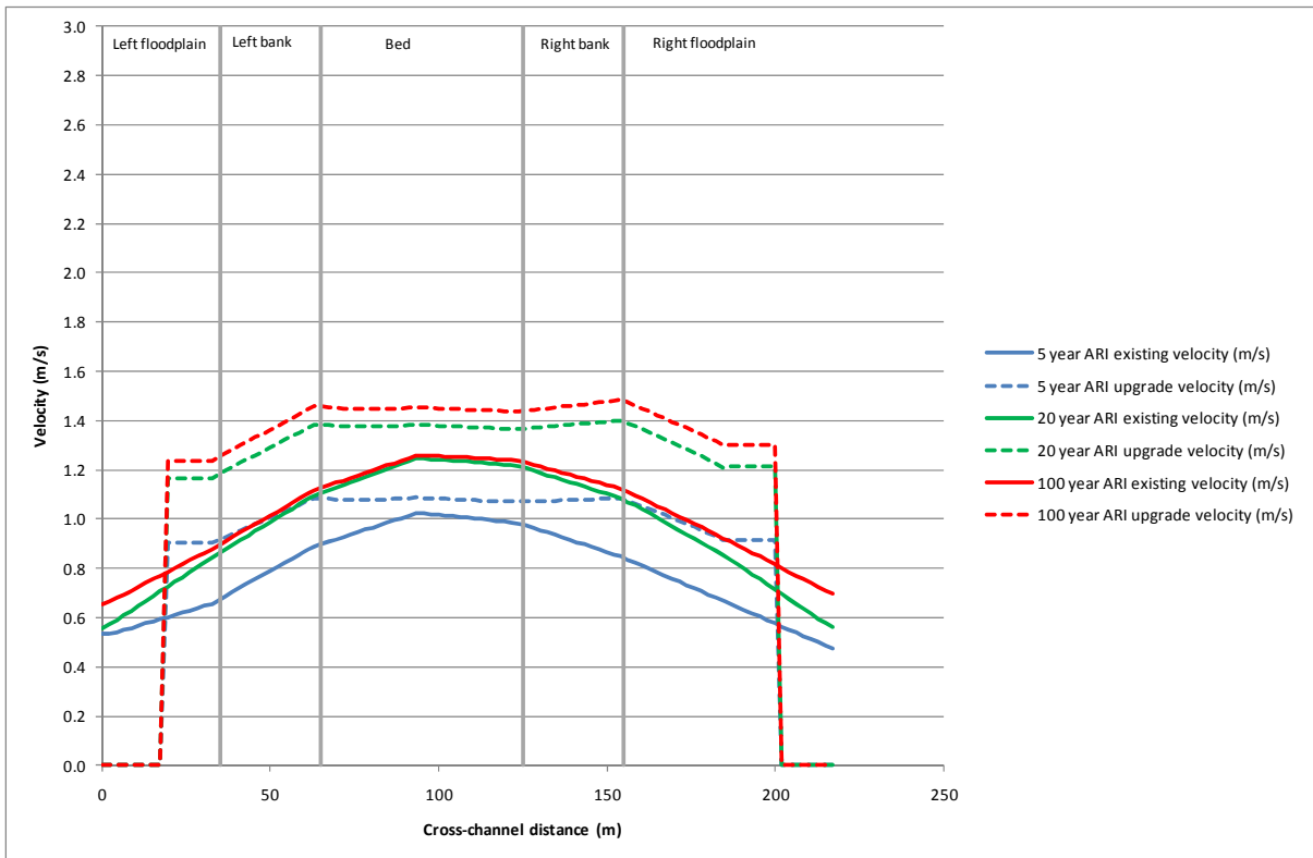
Figure H-18 Velocity profile of Mororo Bridge at station 93.99
