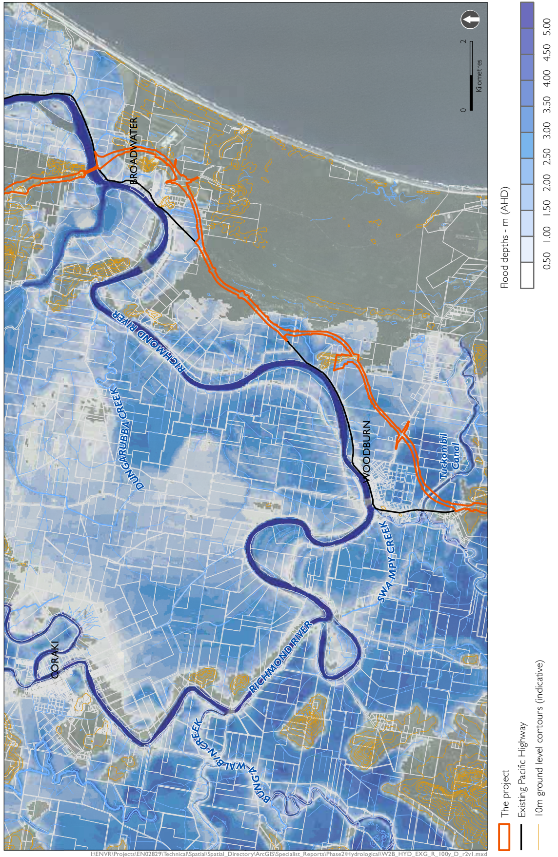
Figure 4-37 Peak 20 year ARI flood depths: Mid Richmond River
