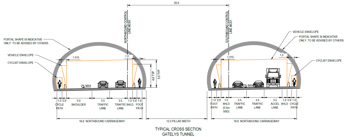
Figure 2-4 Tunnel cross section for the Gatelys Road Tunnel (subject to detailed design)
