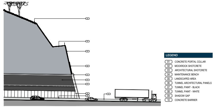
Tunnel portals – typical section
