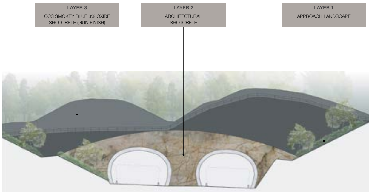
Tunnel portal design approach and materials
